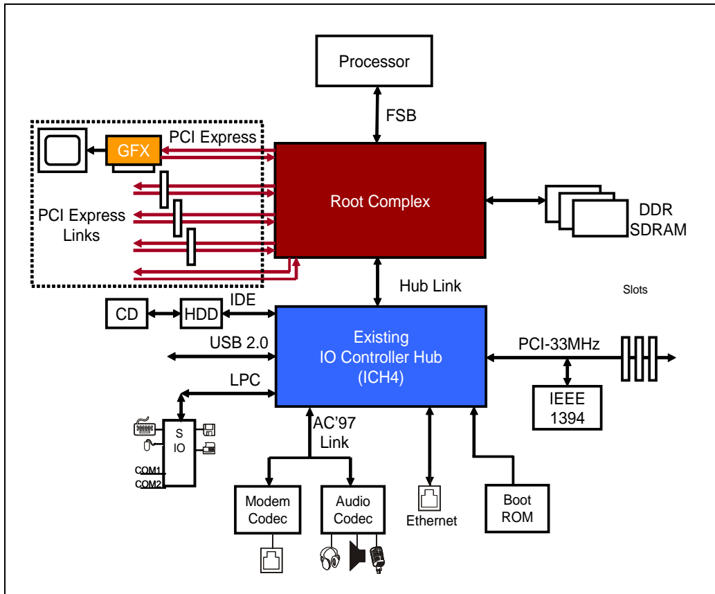
Figure 5: Another Low Cost PCI Express System
